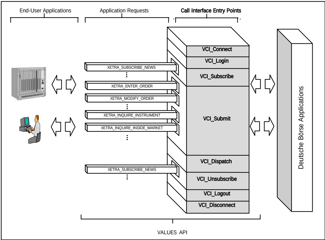
Figure 4.1 - The VALUES API Applications Requests
