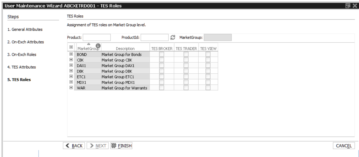
Fig. 97: Screenshot of the User Maintenance Wizard showing the TES roles tab
