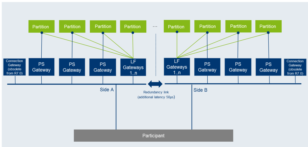
Figure 18: Xetra ETI gateway infrastructure
