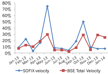
Turnover Velocity
